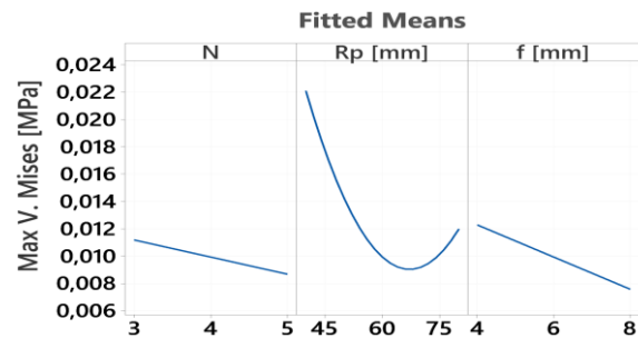
Figure 29. Variation of von Mises stress with response variables for slotted grain.
