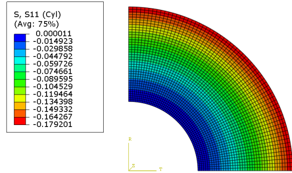
Figure 13. Finite element analysis results of the validation case, radial stress distribution (MPa).
