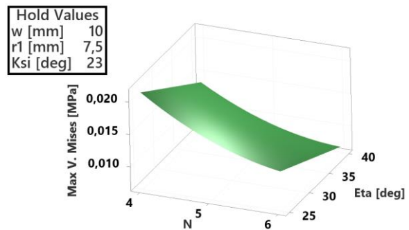
Figure 23. Variation of von Mises stress with N and \eta for star grain.
