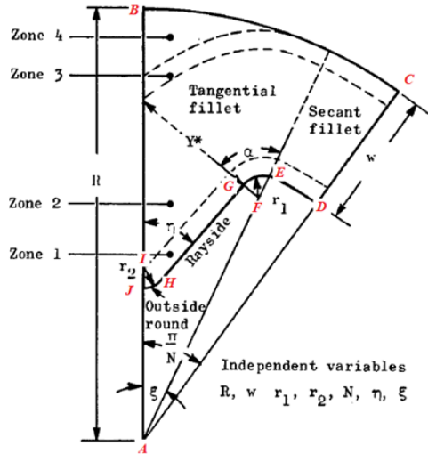
Figure 4. Cross-section parameters of star grains adopted from [9].
