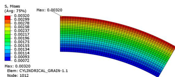
Figure 14. Sample finite element analysis result of tubular grain (for high volumetric loading fraction, r_i=20 mm) (MPa).
