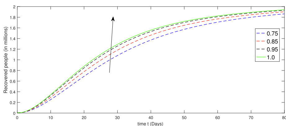
Fig. 5 Dynamical behavior of recovered class (population) for the considered model (2) corresponding to different fraction order derivative.
