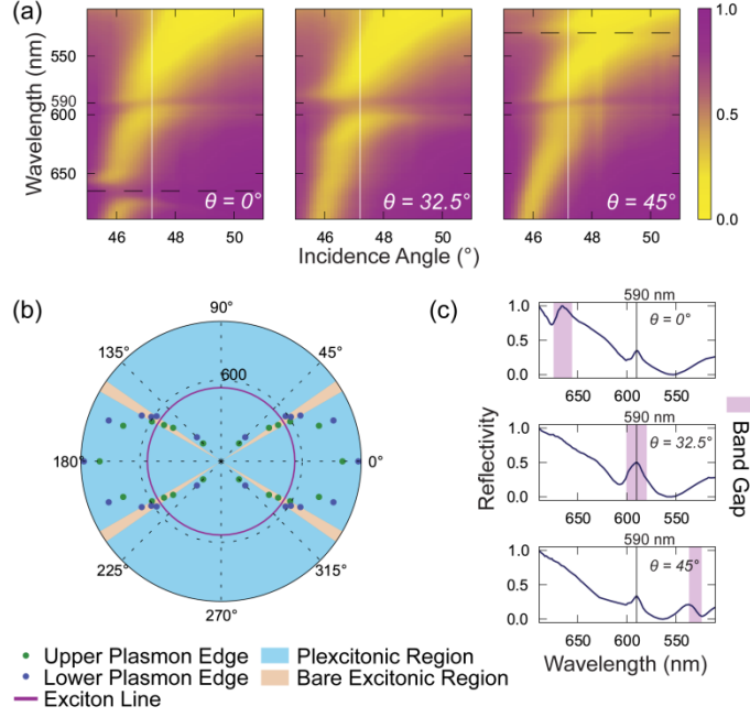
Fig. 2. Experimental realization of 1D plexcitonic crystal with 280 nm pitch with sinus profile. Grating depth is 22 \text{ nm} \pm 1 \text{ nm} . (a) shows experimental reflection maps, confirming the formation of the plexcitons. Anti-crossing behavior (indicated with solid black line) in the reflection map disappears once the absorption line of TDBC dye is introduced inside the band gap of the plasmonic crystal at 32.5^\circ azimuth. (b) shows directional dependence of plexcitonic and bare excitonic regions. Exciton line intersects the band gap separation at 32.5^\circ azimuth angle. SPP-exciton interaction is significantly weak between 30^\circ and 35^\circ azimuth. In (c), this effect is more pronounced. Band gap separation shifts from around 630 nm to 530 nm. At 32.5^\circ azimuth angle, TDBC absorption line is totally inside the band gap.
